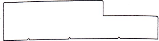
1-5/16 X 5-1/4 SINGLE RABBETED EXTERIOR JAMB *PRIMED
