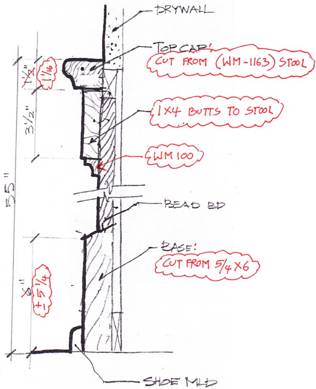
WAINSCOT DETAIL SCALE: NTS
